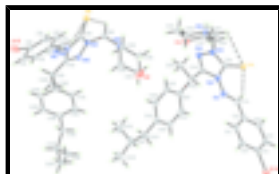
Fig. 1. The asymmetric unit of the title compound. Displacement ellipsoids are drawn at the 50% probability level. Hydrogen bonds are shown as dashed lines.
