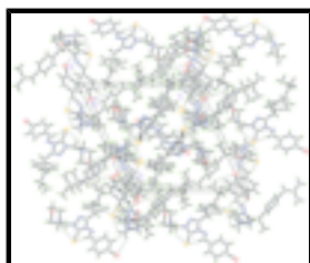
Fig. 2. The crystal packing of the title compound, viewed along the a axis. Hydrogen bonds are shown as dashed lines.
